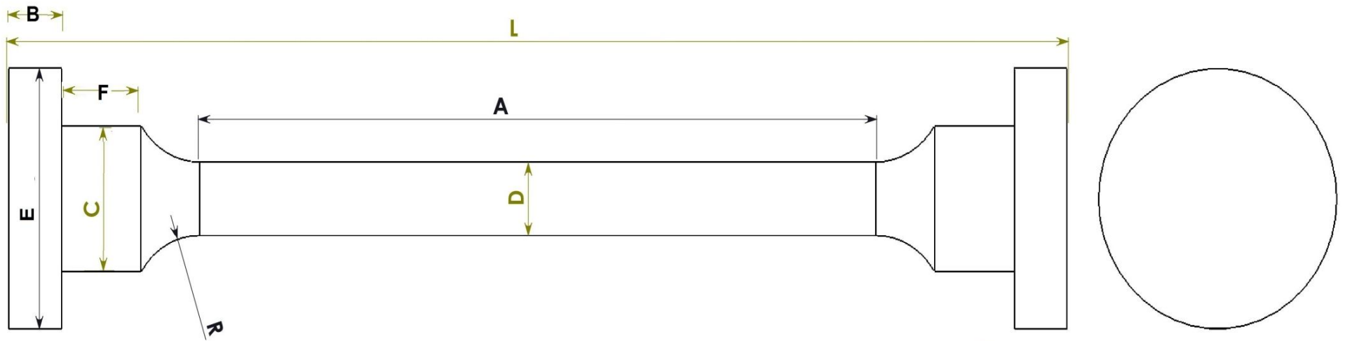
Tensile Test Specimen (Round Sub-size)
